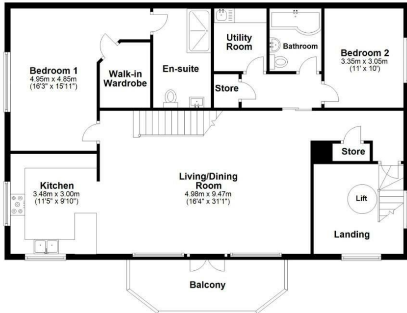
First Floor Approx. 126.3 sq. metres (1359.6 sq. feet)
